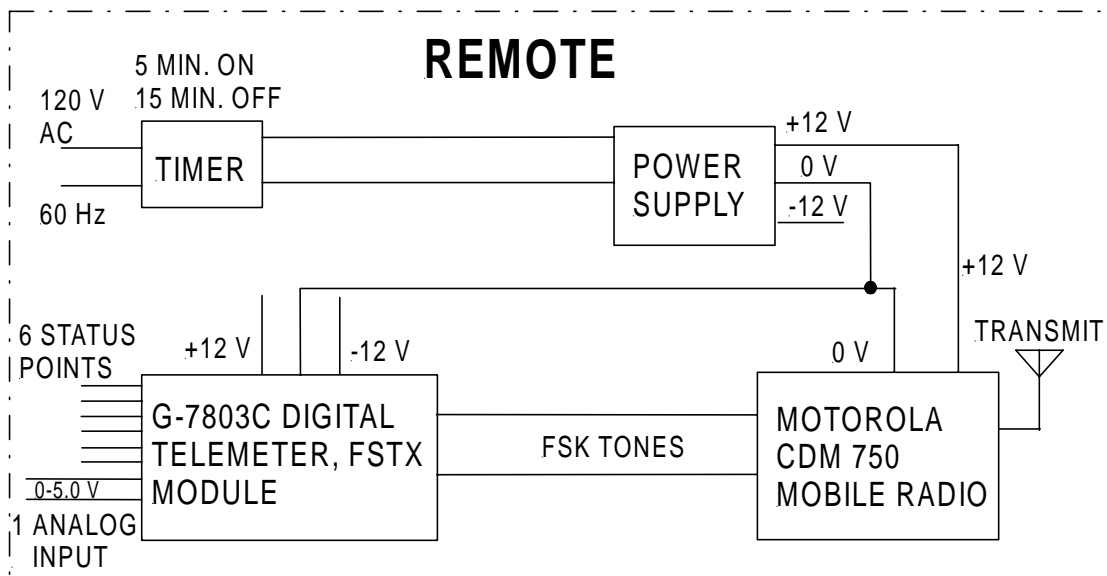
APPLICATION BLOCK DIAGRAM FOR DIGITAL TELEMETERS AND RADIO
